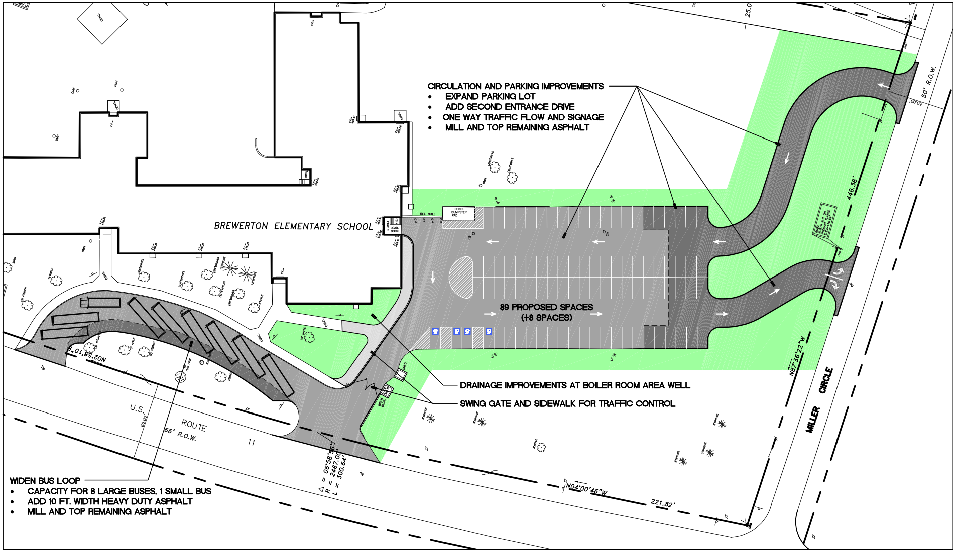
CENTRAL SQUARE CSD BREWERTON ELEMENTARY SITE SCHEMATIC SK-2
